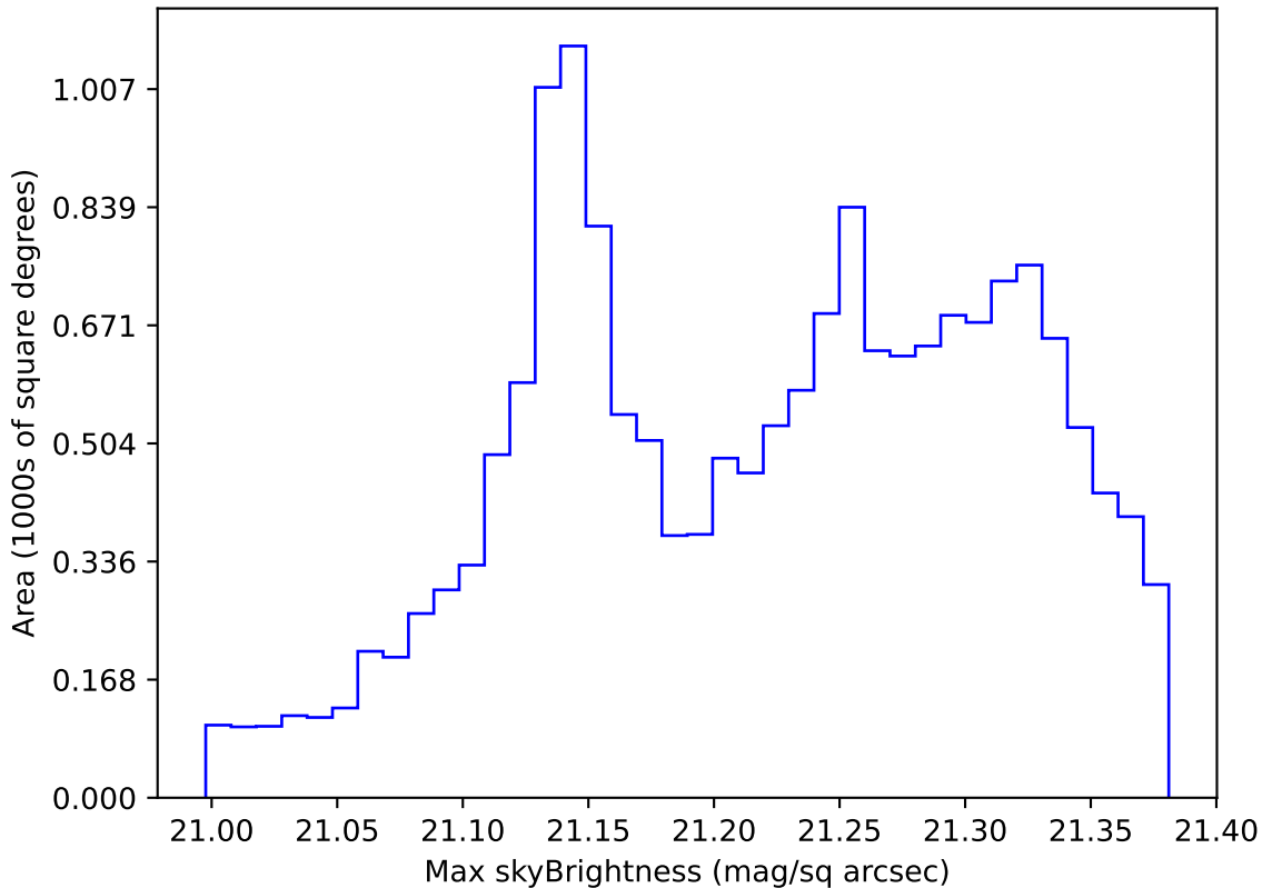
ddf_acor_sf15_lsf20_lsr20_v3.4_10yrs WFD r band: Max skyBrightness
