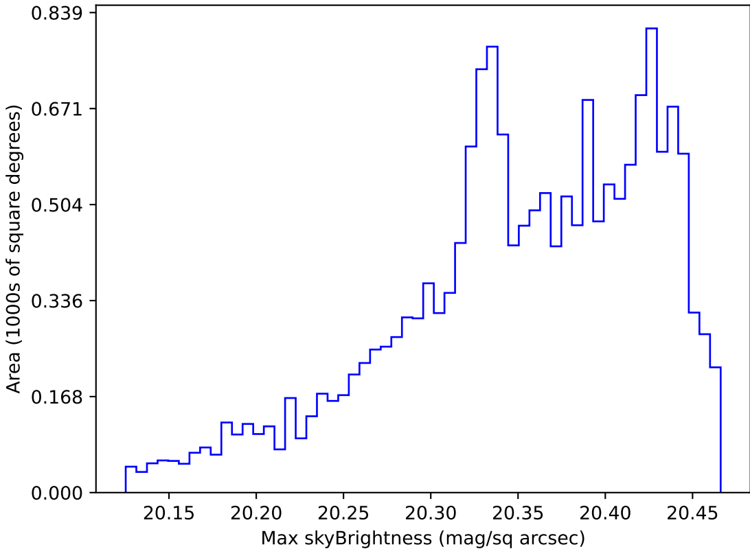
ddf_acor_sf15_lsf20_lsr20_v3.4_10yrs WFD i band: Max skyBrightness
