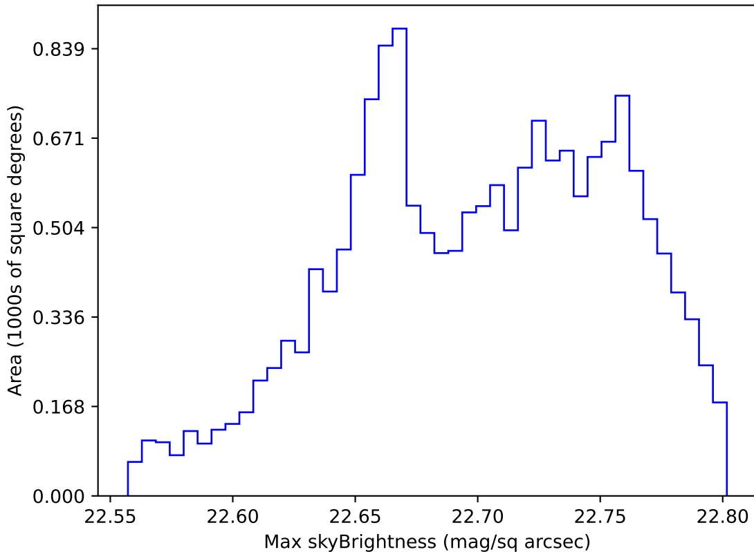
ddf_acor_sf15_lsf20_lsr20_v3.4_10yrs WFD all bands: Max skyBrightness
