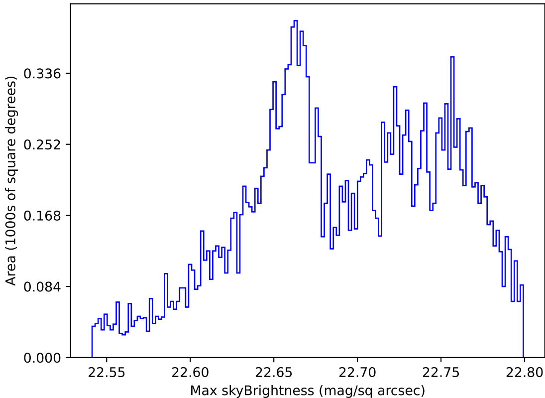
ddf_acor_sf15_lsf20_lsr20_v3.4_10yrs All sky u band: Max skyBrightness
