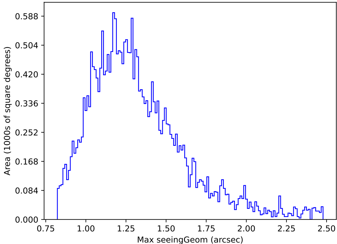
ddf_acor_sf15_lsf20_lsr20_v3.4_10yrs Yr 1 z band: Max seeingGeom
