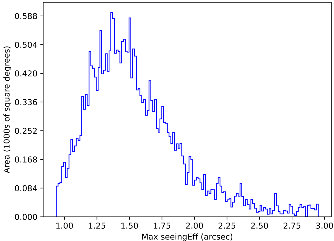
ddf_acor_sf15_lsf20_lsr20_v3.4_10yrs Yr 1 z band: Max seeingEff
