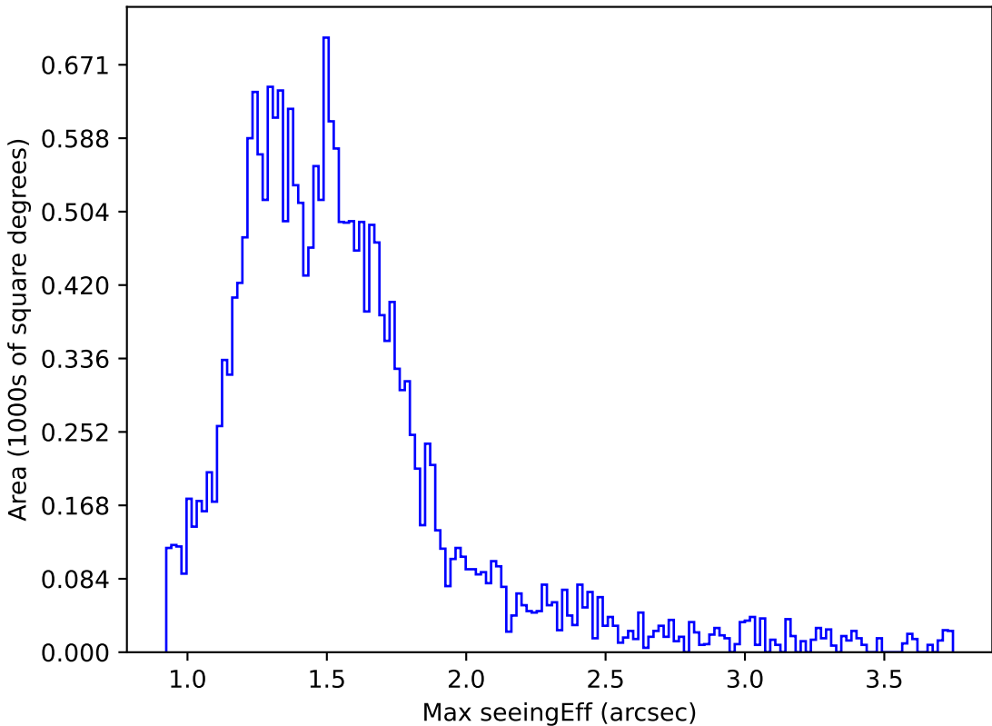
ddf_acor_sf15_lsf20_lsr20_v3.4_10yrs Yr 1 u band: Max seeingEff
