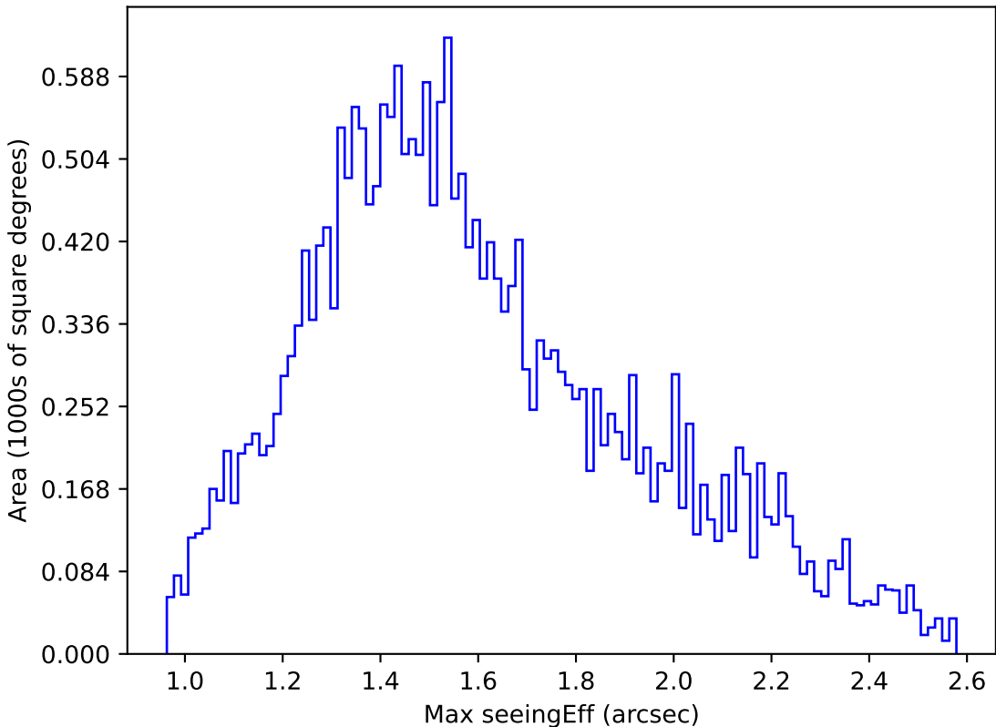
ddf_acor_sf15_lsf20_lsr20_v3.4_10yrs Yr 1 r band: Max seeingEff
