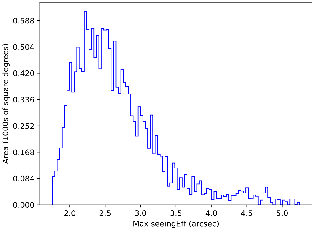
ddf_acor_sf15_lsf20_lsr20_v3.4_10yrs WFD z band: Max seeingEff
