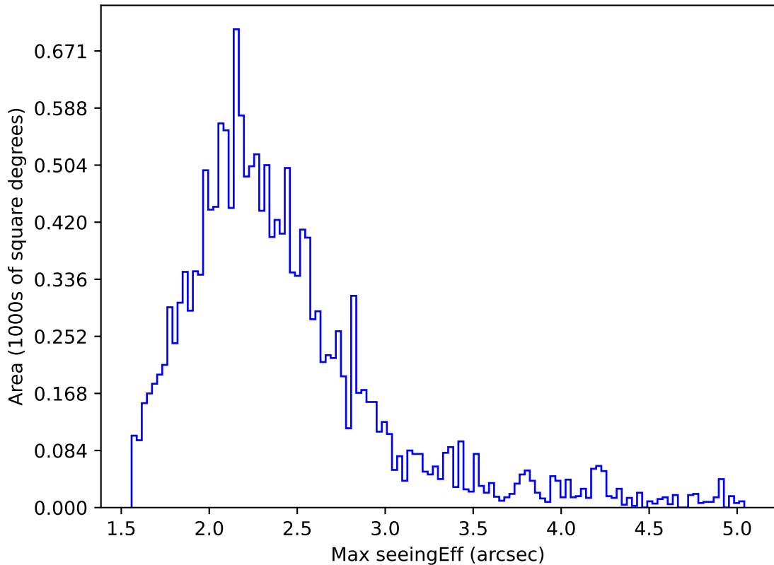
ddf_acor_sf15_lsf20_lsr20_v3.4_10yrs WFD y band: Max seeingEff
