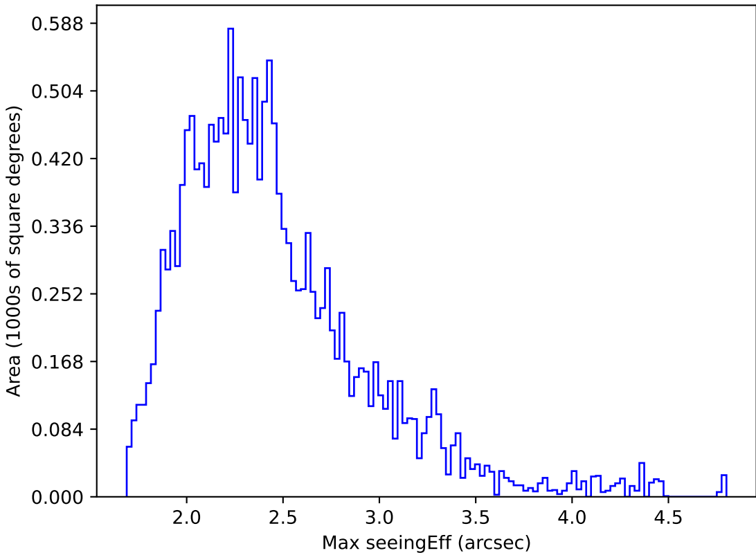
ddf_acor_sf15_lsf20_lsr20_v3.4_10yrs WFD u band: Max seeingEff
