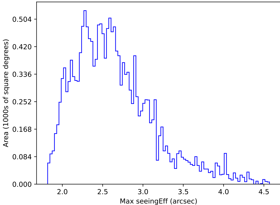
ddf_acor_sf15_lsf20_lsr20_v3.4_10yrs WFD r band: Max seeingEff
