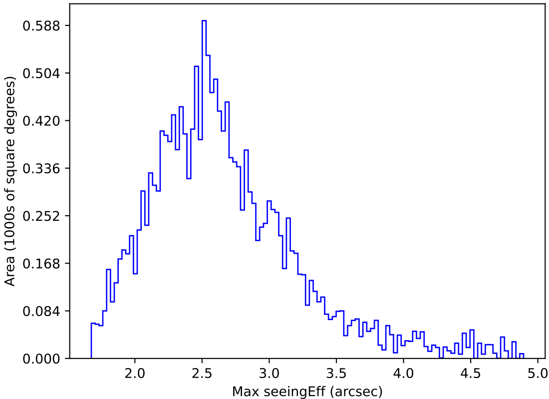
ddf_acor_sf15_lsf20_lsr20_v3.4_10yrs WFD i band: Max seeingEff
