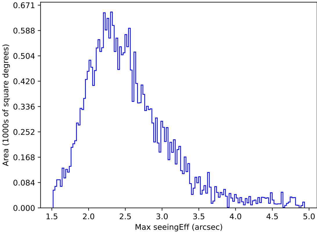
ddf_acor_sf15_lsf20_lsr20_v3.4_10yrs All sky z band: Max seeingEff
