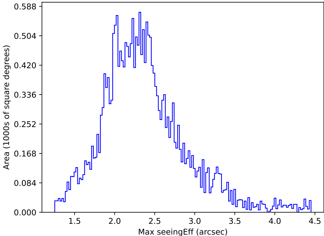
ddf_acor_sf15_ls20_lsr20_v3.4_10yrs All sky u band: Max seeingEff
