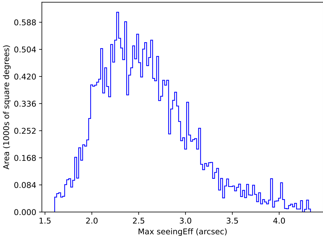
ddf_acor_sf15_lsf20_lsr20_v3.4_10yrs All sky r band: Max seeingEff
