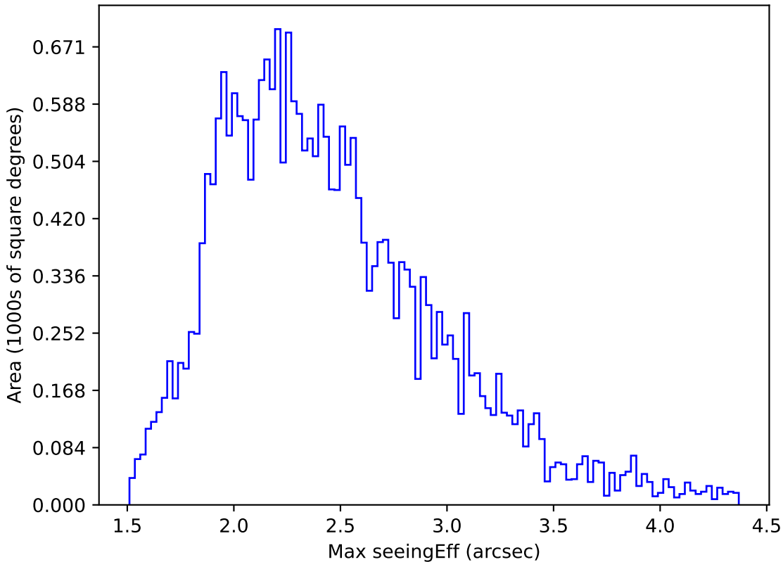
ddf_acor_sf15_ls20_lsr20_v3.4_10yrs All sky g band: Max seeingEff
