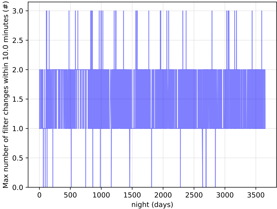
ddf_acor_sf15_Isf20_Isr20_v3.4_10yrs Per Night: Max number of filter changes within 10.0 minutes
