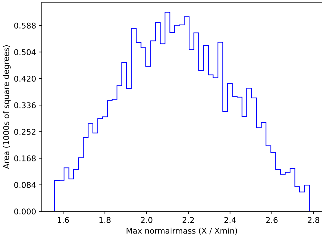
ddf_acor_sf15_lsf20_lsr20_v3.4_10yrs WFD y band: Max normairmass
