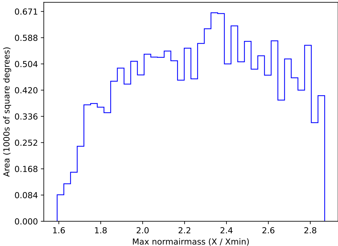
ddf_acor_sf15_lsf20_lsr20_v3.4_10yrs WFD i band: Max normairmass
