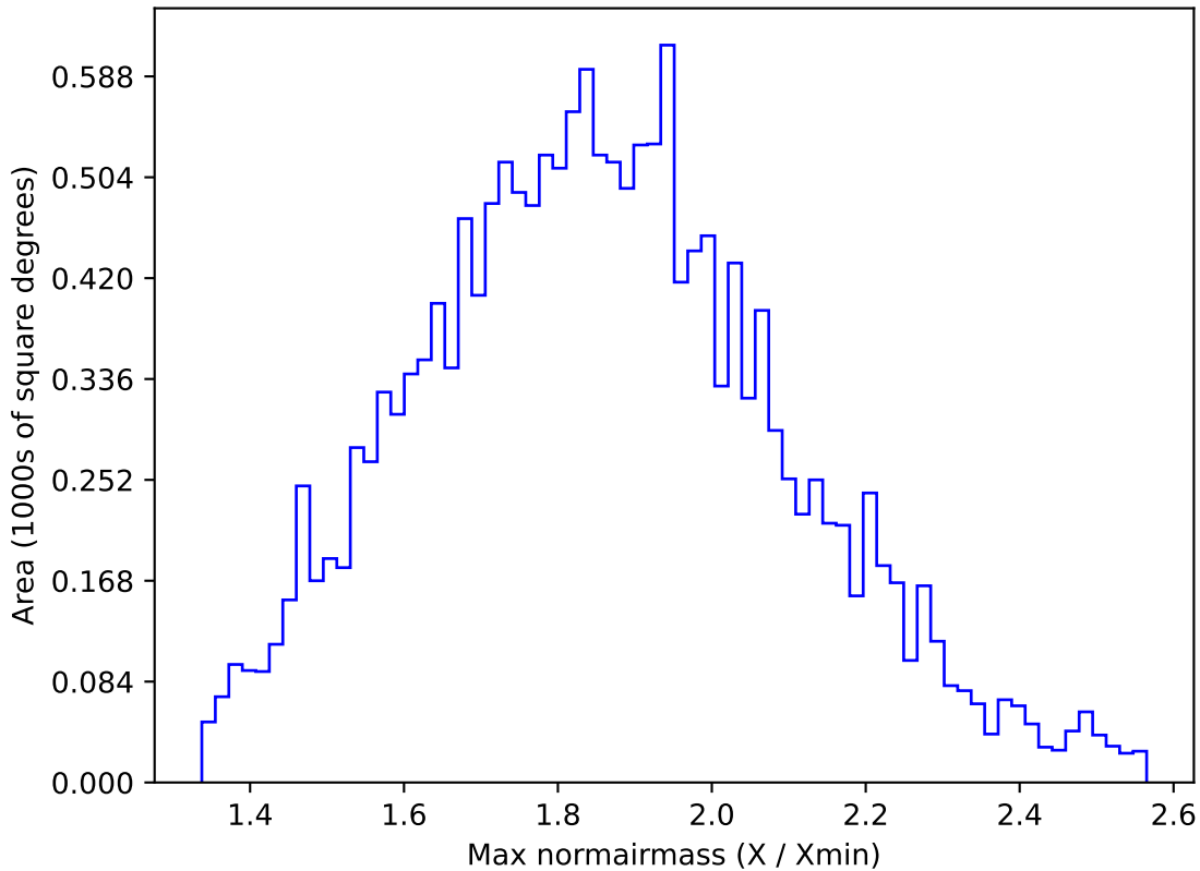
ddf_acor_sf15_lsf20_lsr20_v3.4_10yrs WFD g band: Max normairmass
