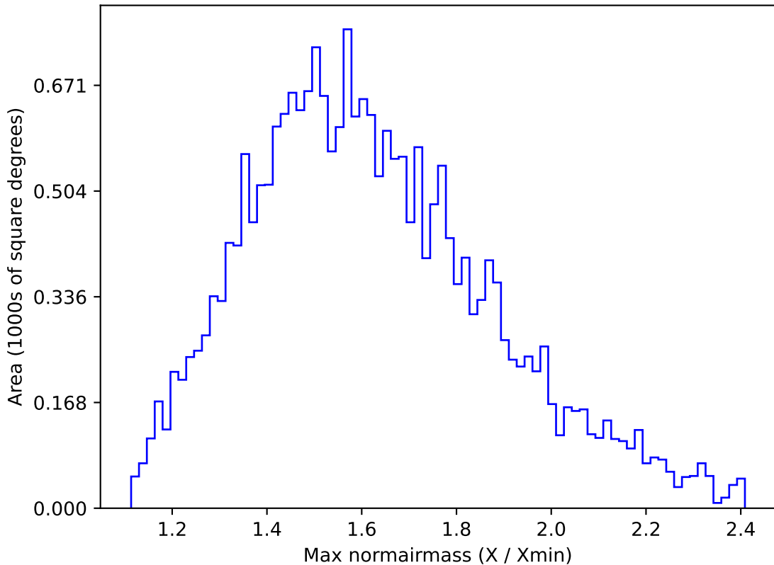
ddf_acor_sf15_lsf20_lsr20_v3.4_10yrs All sky u band: Max normairmass
