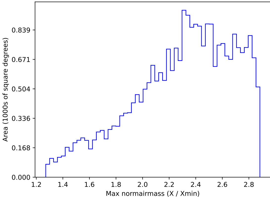
ddf_acor_sf15_lsf20_lsr20_v3.4_10yrs All sky all bands: Max normairmass
