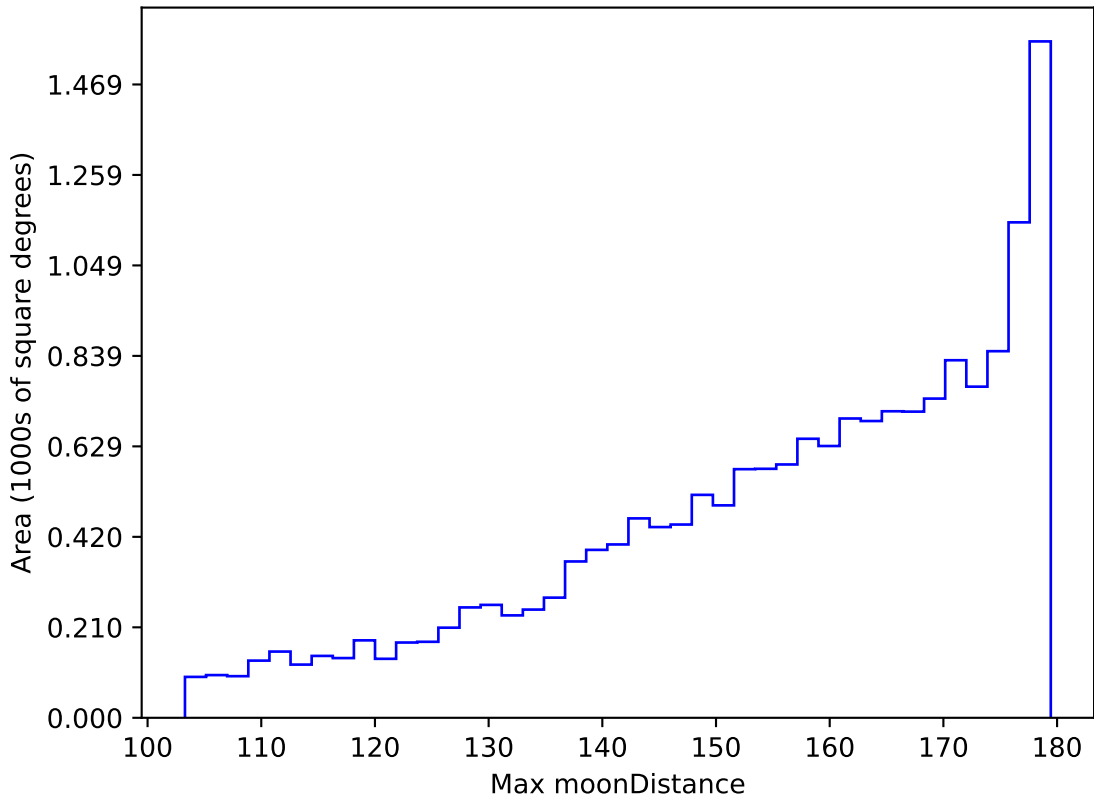
ddf_acor_sf15_lsf20_lsr20_v3.4_10yrs WFD r band: Max moonDistance
