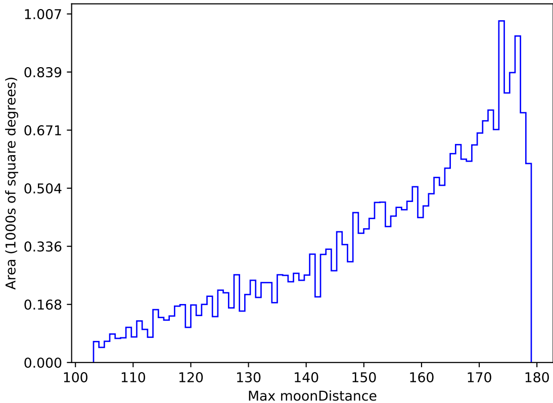
ddf_acor_sf15_lsf20_lsr20_v3.4_10yrs All sky g band: Max moonDistance
