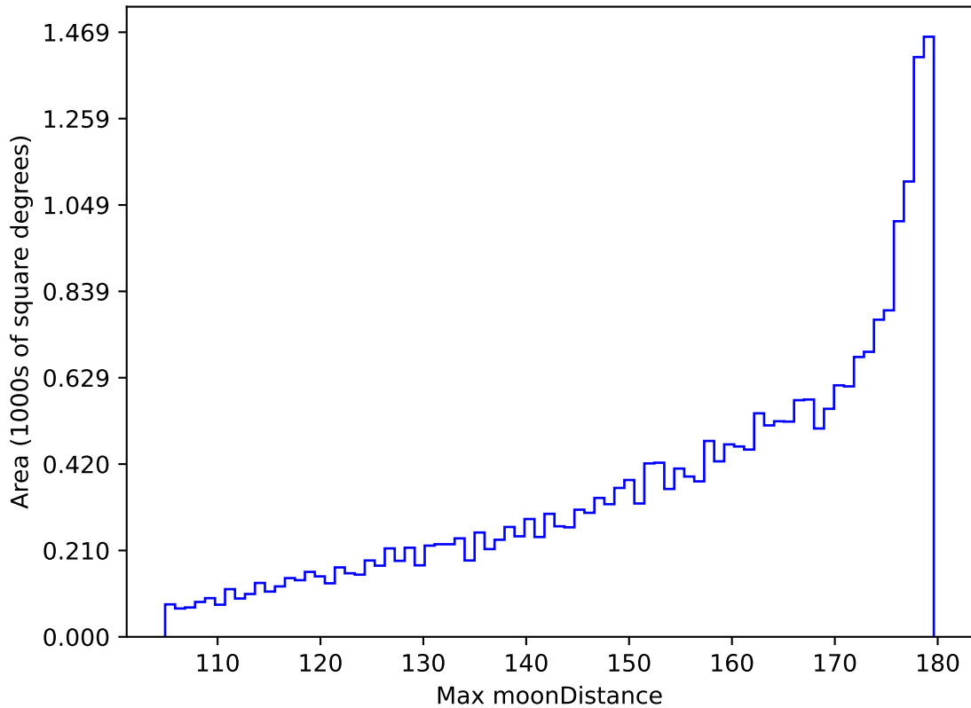
ddf_acor_sf15_lsf20_lsr20_v3.4_10yrs All sky all bands: Max moonDistance
