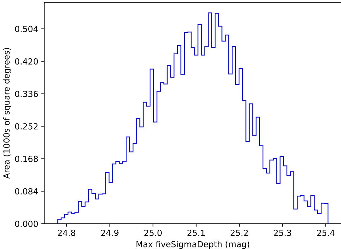
ddf_acor_sf15_lsf20_lsr20_v3.4_10yrs WFD all bands: Max fiveSigmaDepth
