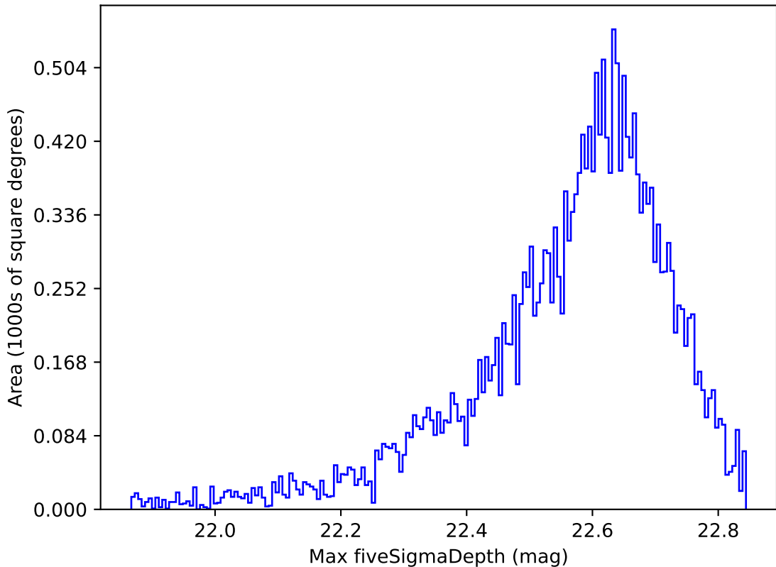
ddf_acor_sf15_ls20_lsr20_v3.4_10yrs All sky y band: Max fiveSigmaDepth
