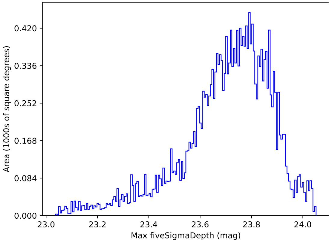
ddf_acor_sf15_ls20_lsr20_v3.4_10yrs All sky u band: Max fiveSigmaDepth
