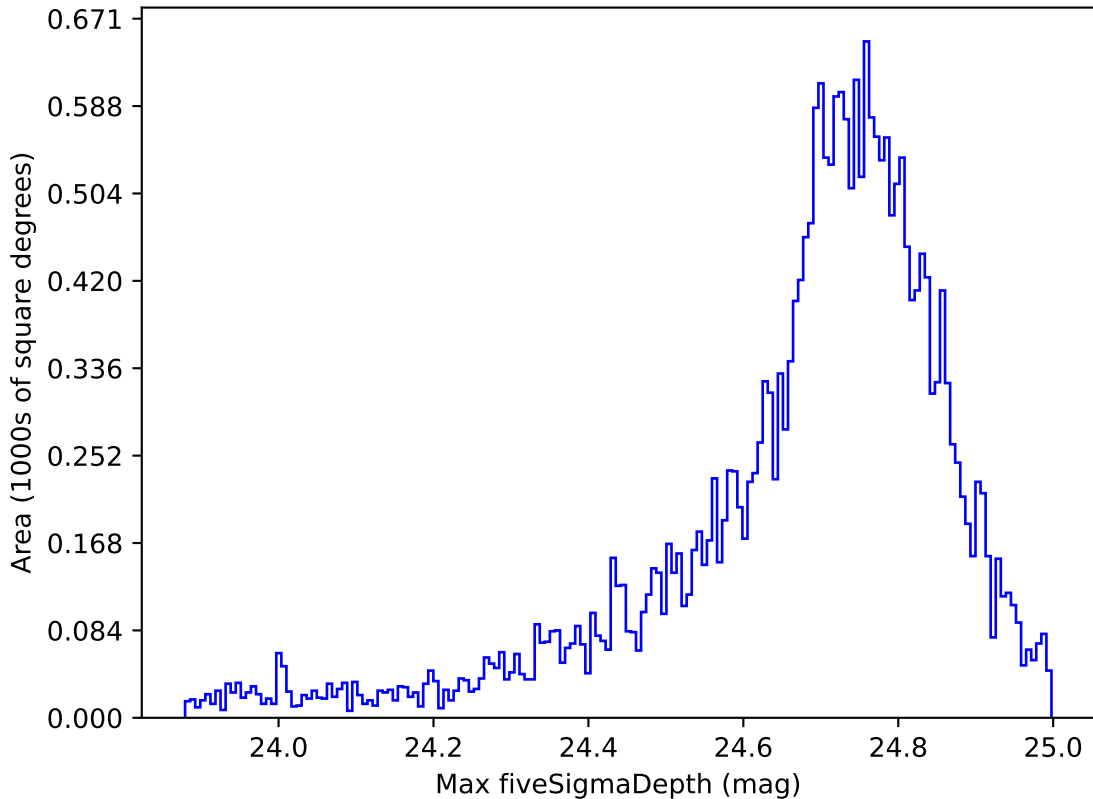
ddf_acor_sf15_lsf20_lsr20_v3.4_10yrs All sky r band: Max fiveSigmaDepth
