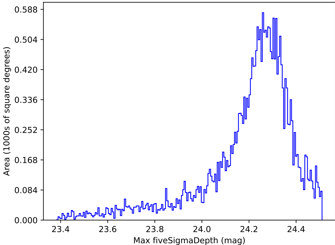
ddf_acor_sf15_lsf20_lsr20_v3.4_10yrs All sky i band: Max fiveSigmaDepth
