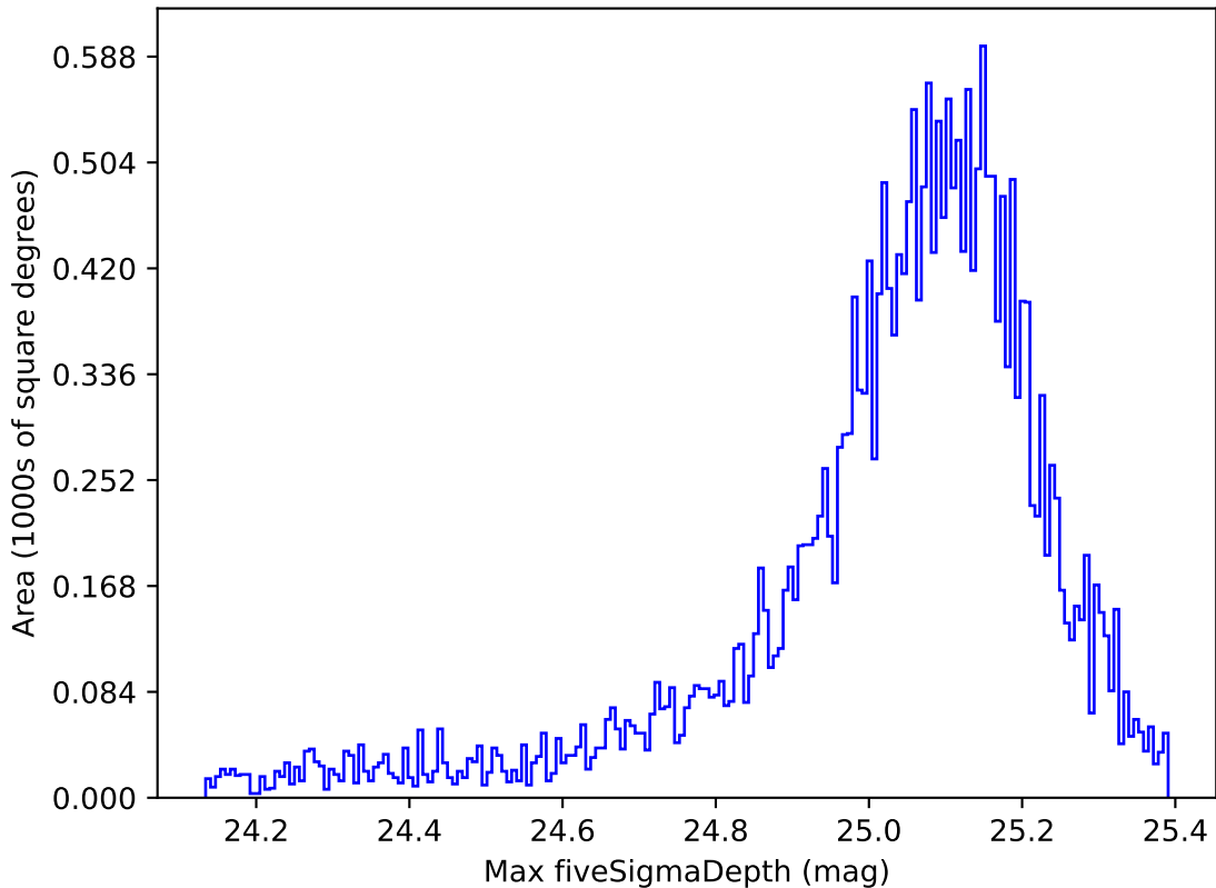
ddf_acor_sf15_ls20_lsr20_v3.4_10yrs All sky g band: Max fiveSigmaDepth
