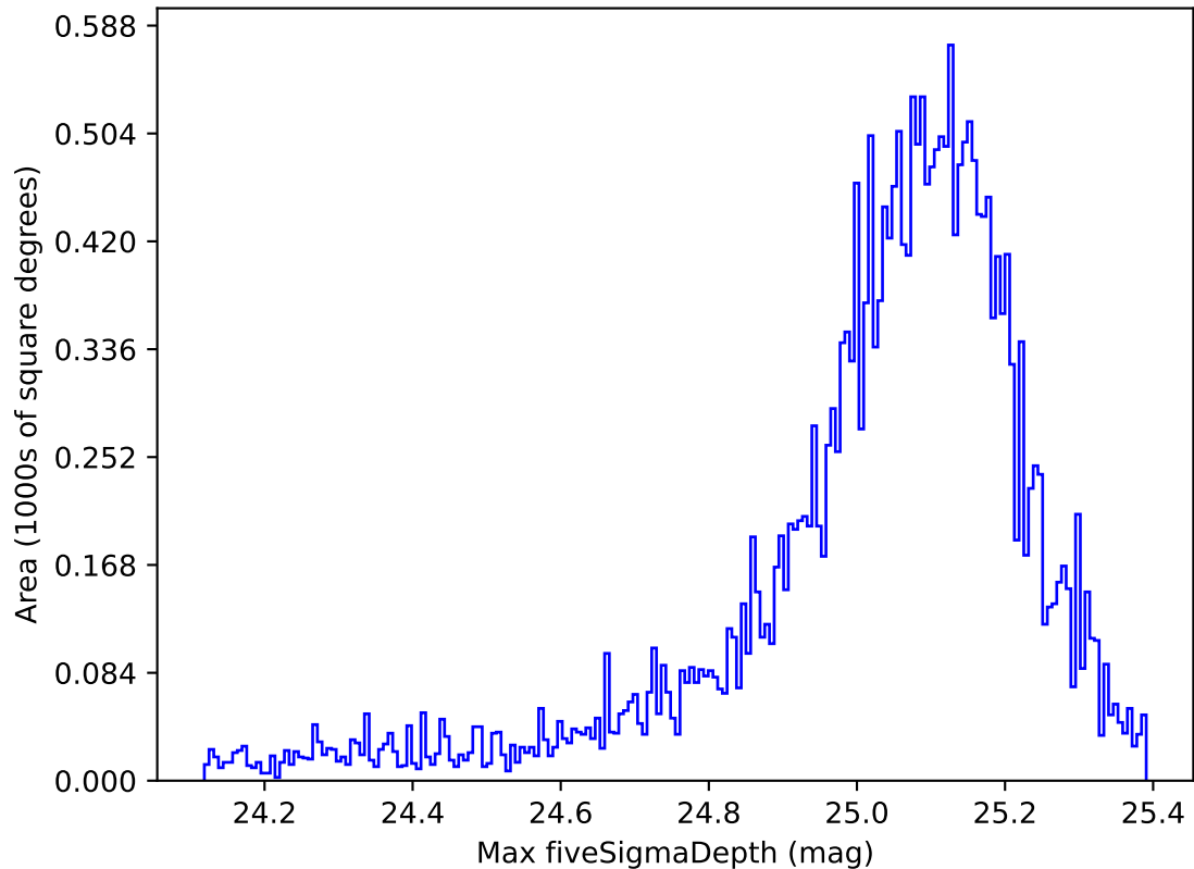
ddf_acor_sf15_lsf20_lsr20_v3.4_10yrs All sky all bands: Max fiveSigmaDepth
