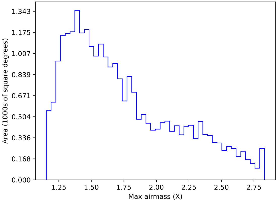
ddf_acor_sf15_lsf20_lsr20_v3.4_10yrs Yr 1 z band: Max airmass
