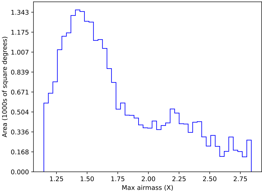
ddf_acor_sf15_lsf20_lsr20_v3.4_10yrs Yr 1 i band: Max airmass
