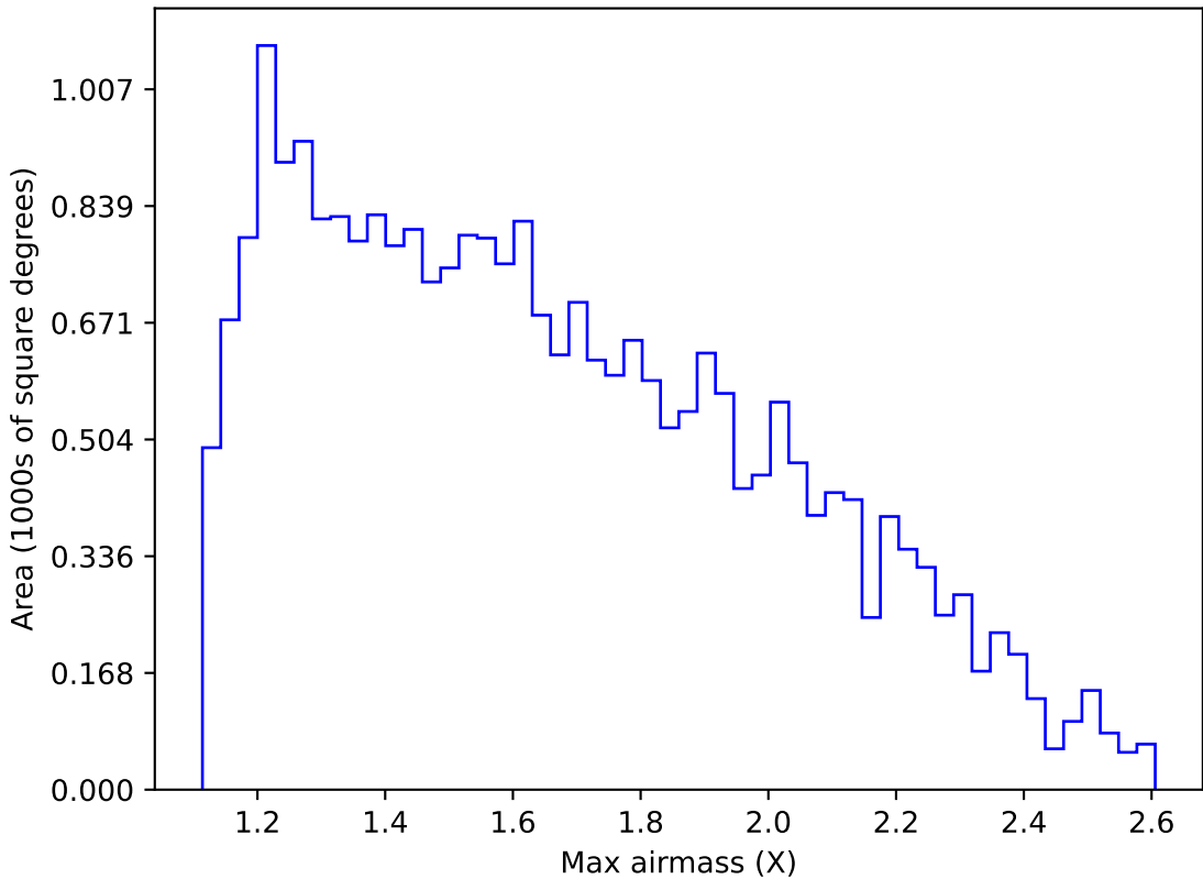
ddf_acor_sf15_lsf20_lsr20_v3.4_10yrs Yr 1 g band: Max airmass
