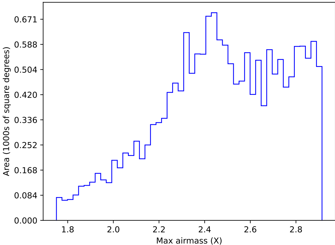
ddf_acor_sf15_lsf20_lsr20_v3.4_10yrs WFD z band: Max airmass
