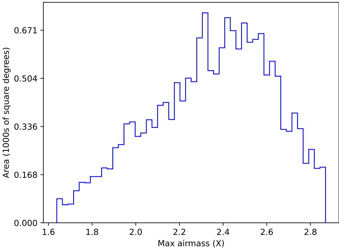
ddf_acor_sf15_ls20_lsr20_v3.4_10yrs WFD y band: Max airmass
