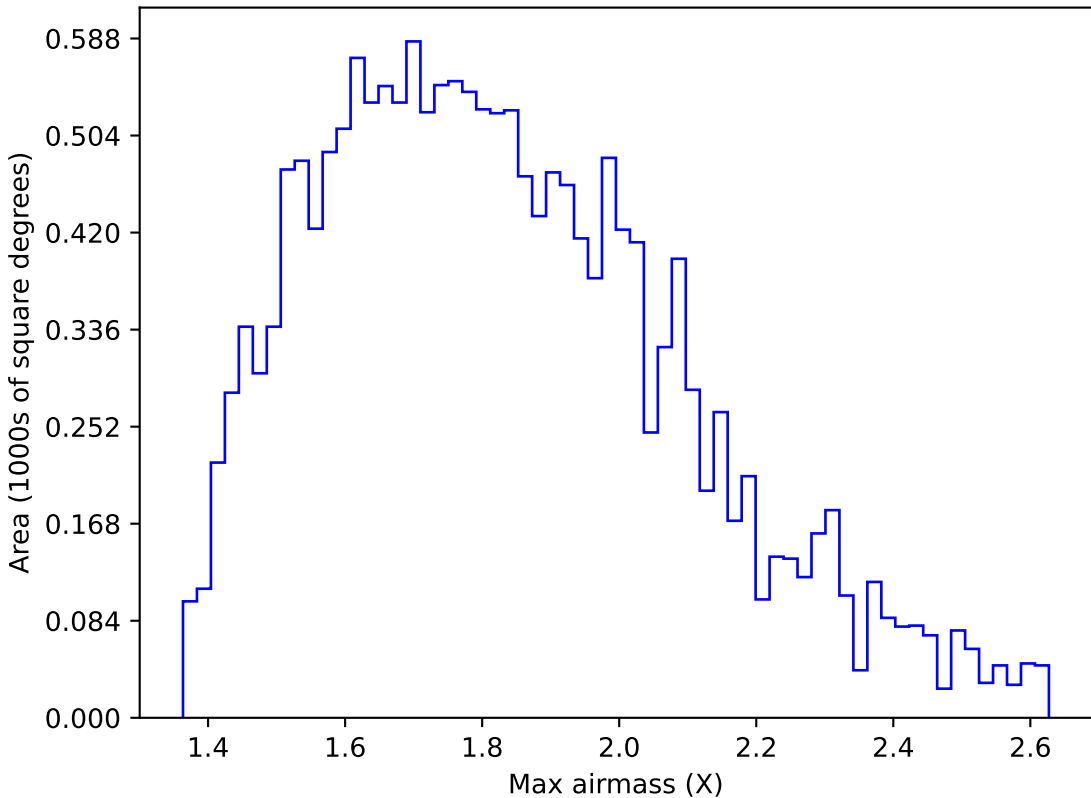
ddf_acor_sf15_lsf20_lsr20_v3.4_10yrs WFD u band: Max airmass
