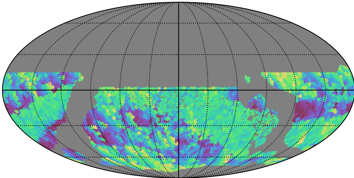
ddf_acor_sf15_lsf20_lsr20_v3.4_10yrs WFD r band: Max airmass
