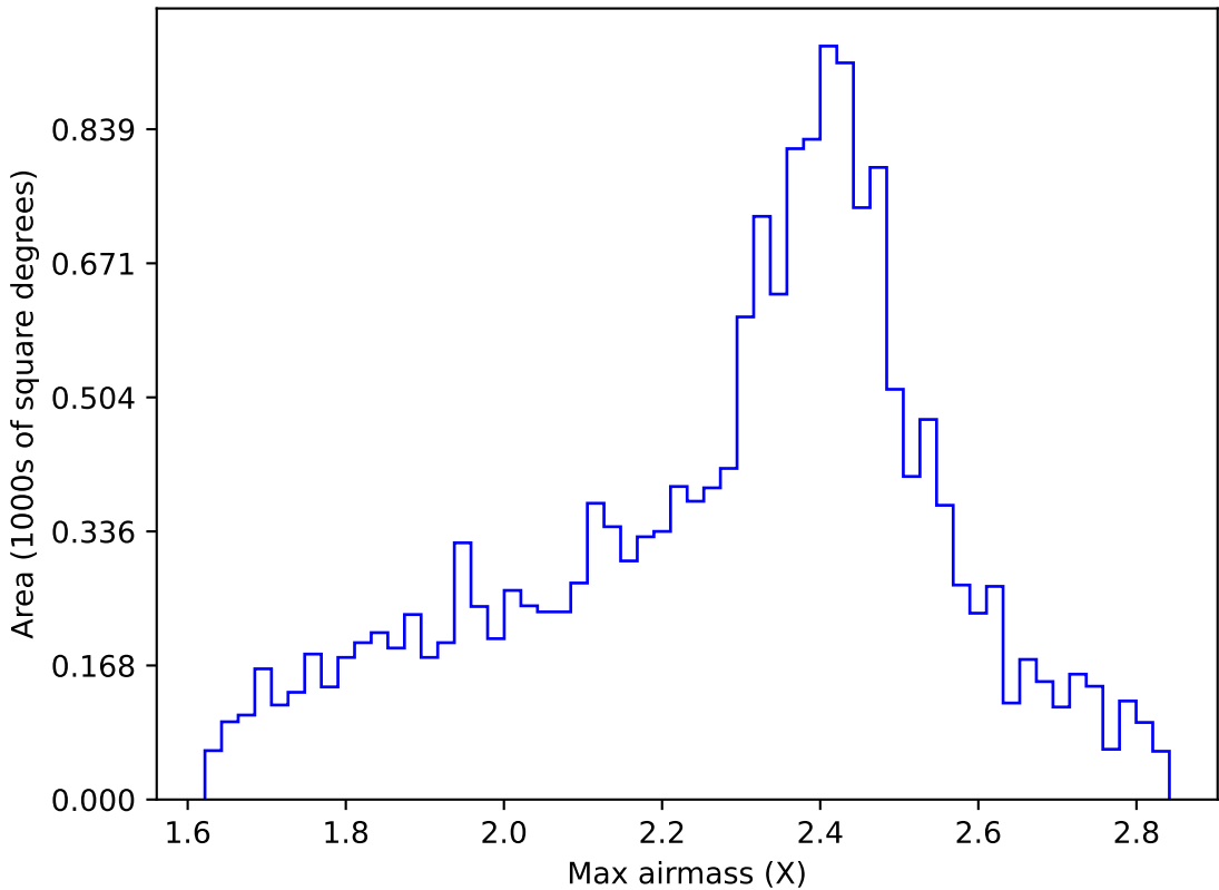
ddf_acor_sf15_lsf20_lsr20_v3.4_10yrs WFD r band: Max airmass
