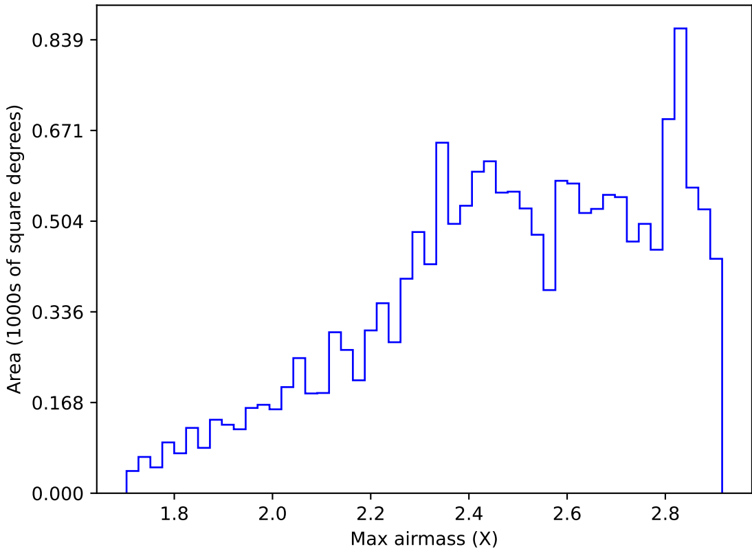
ddf_acor_sf15_lsf20_lsr20_v3.4_10yrs WFD i band: Max airmass
