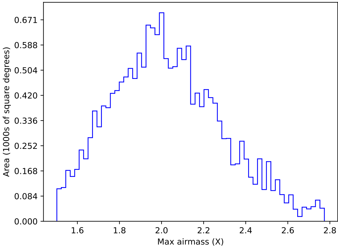
ddf_acor_sf15_lsf20_lsr20_v3.4_10yrs WFD g band: Max airmass
