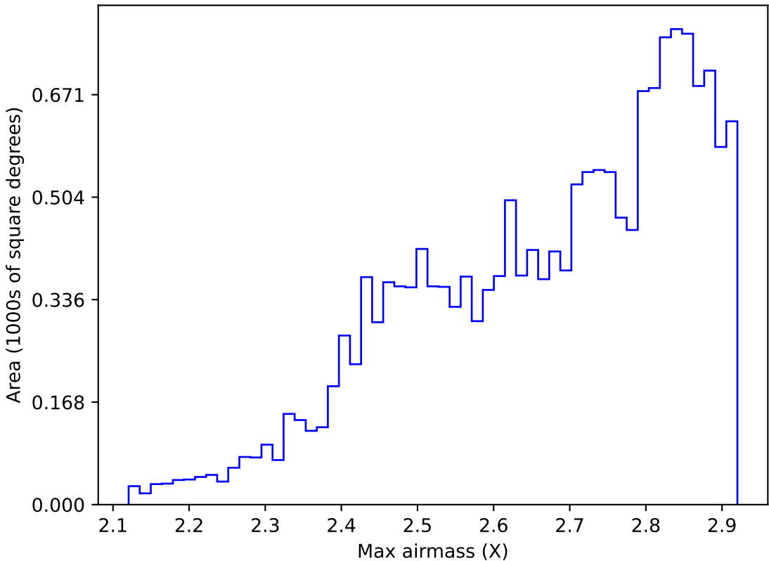
ddf_acor_sf15_lsf20_lsr20_v3.4_10yrs WFD all bands: Max airmass
