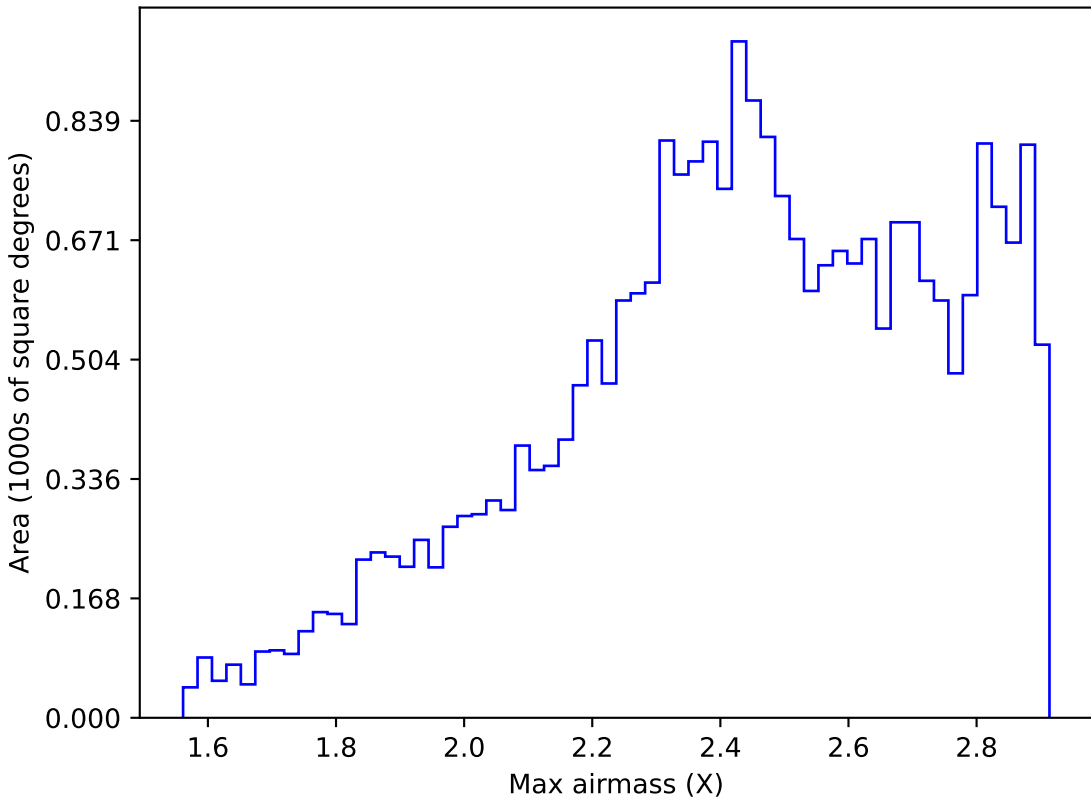
ddf_acor_sf15_lsf20_lsr20_v3.4_10yrs All sky z band: Max airmass
