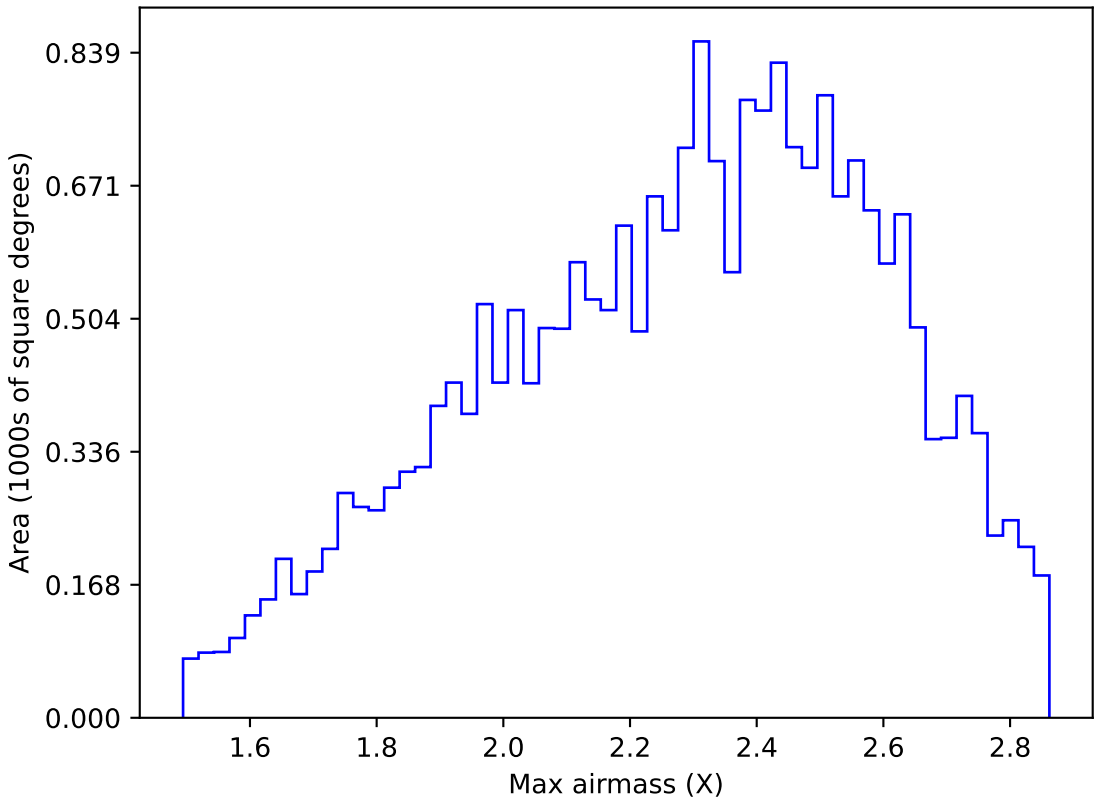
ddf_acor_sf15_lsf20_lsr20_v3.4_10yrs All sky y band: Max airmass
