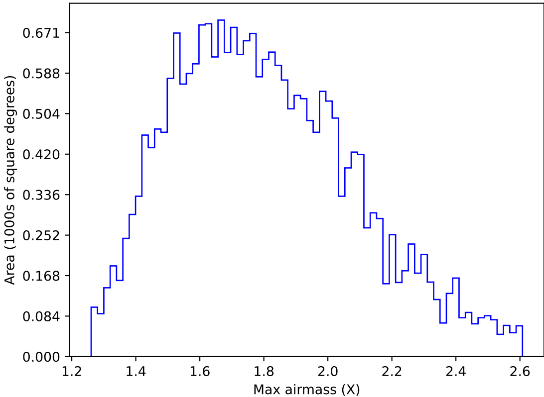
ddf_acor_sf15_lsf20_lsr20_v3.4_10yrs All sky u band: Max airmass
