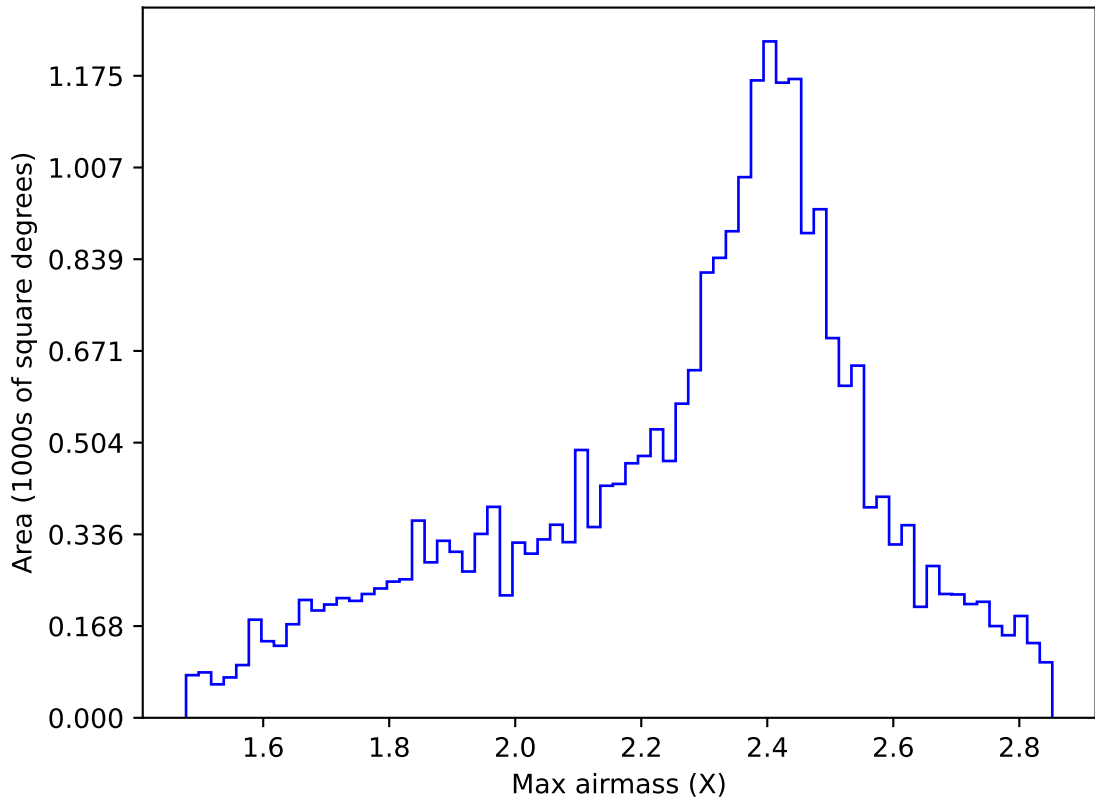
ddf_acor_sf15_lsf20_lsr20_v3.4_10yrs All sky r band: Max airmass
