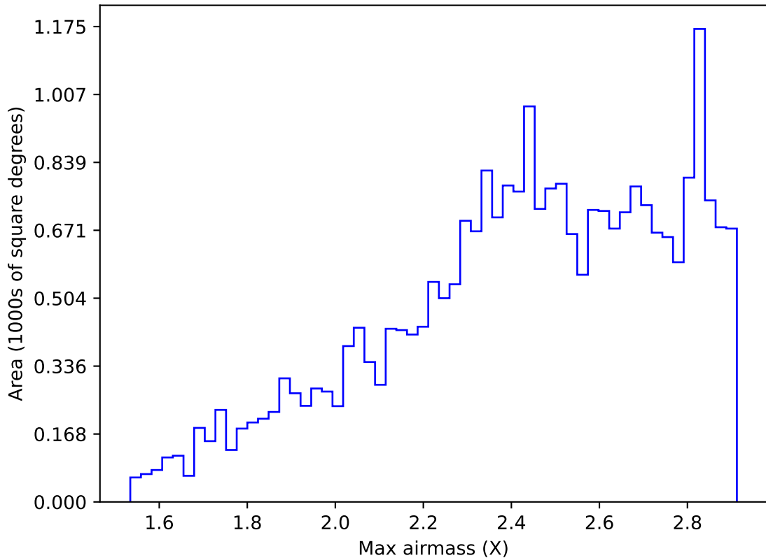
ddf_acor_sf15_lsf20_lsr20_v3.4_10yrs All sky i band: Max airmass
