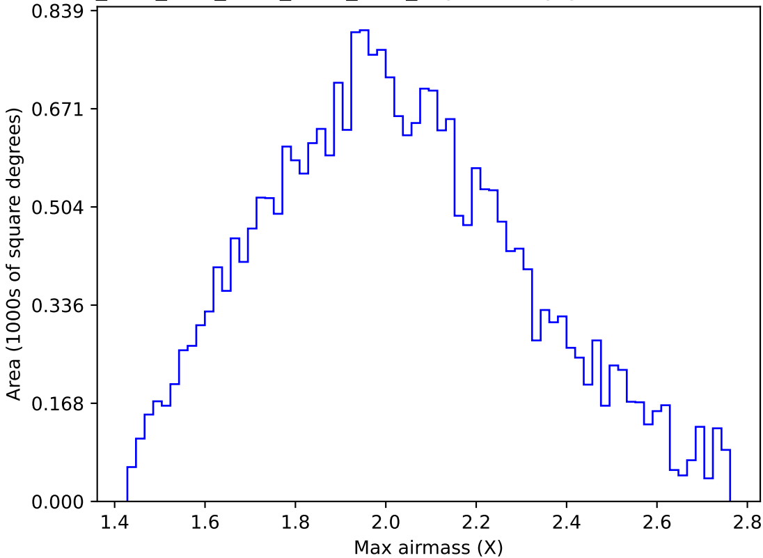
ddf_acor_sf15_lsf20_lsr20_v3.4_10yrs All sky g band: Max airmass
